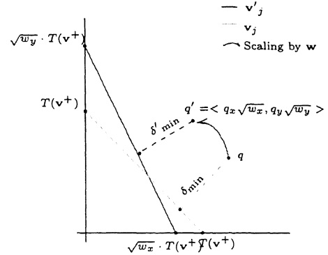
Figure 13: The lower- and upper bound on the Euclidean distance with weighting vector \mathbf{w} , visualized for m = N - 2 .
